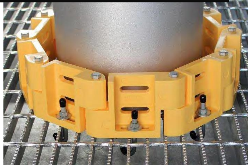
One Link (T5) To Encircle All Pipe Sizes
